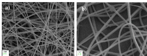
Figure 1: SEM images of PDMS- b -PMMA nanofibers obtained from 1000 g/mol PDMS macroinitiator: a) 0 wt% and b) 8 wt% GO relative to polymer.
