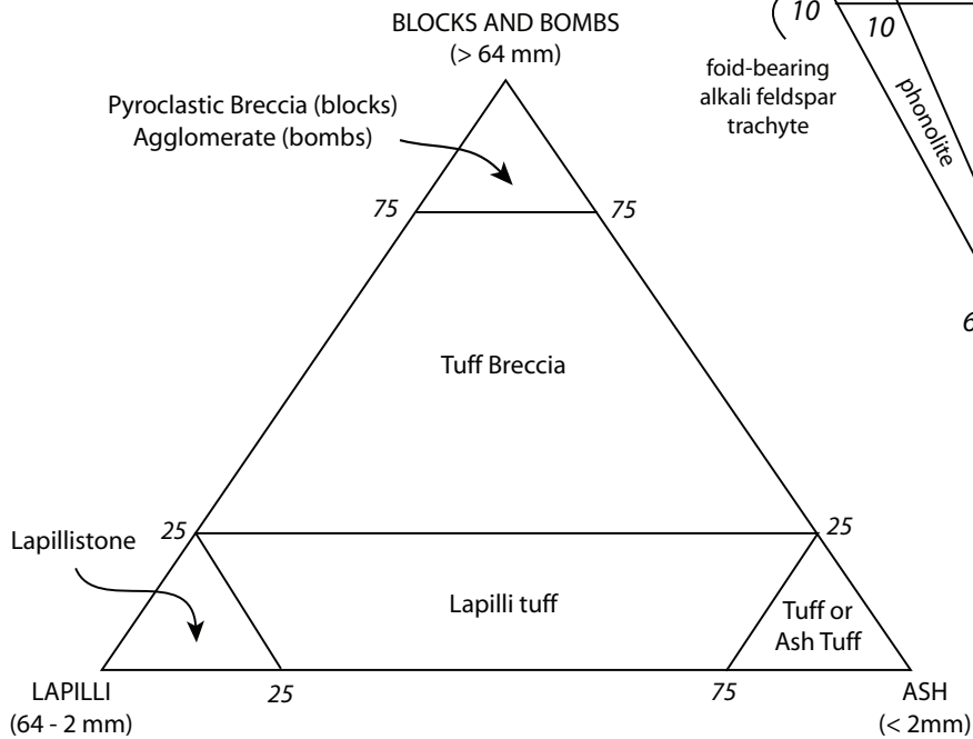
Classification of Pyroclastic Rocks
