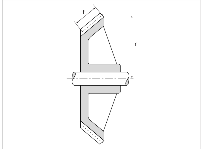
Fig. 8.06 Ribbed bevel gear
