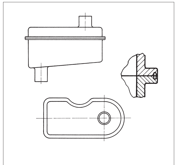
Fig. 10.84 Automotive tank
