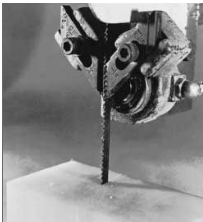
Fig. 11.02 Sawing Machining conditions: Saw speed, 1200 m per min; blade, 6 mm wide, 4 teeth per cm; No coolant. Material – ZYTEL® 101 – 35 mm thick.
