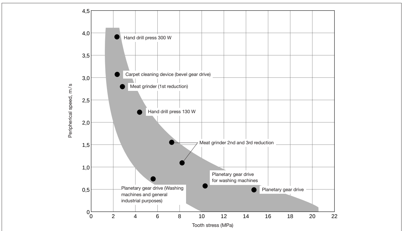
Fig. 8.01 Speed versus stress: Typical gear applications placed on curve
